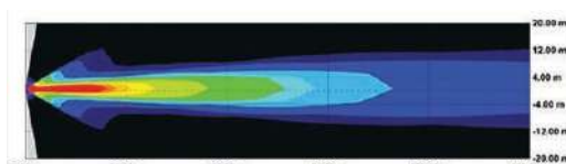
Spot Beam
