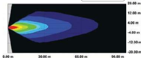
Flood Beam
