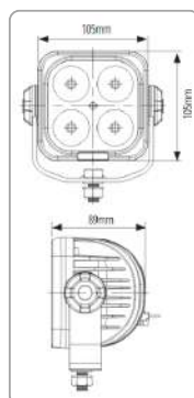
Spot Beam
